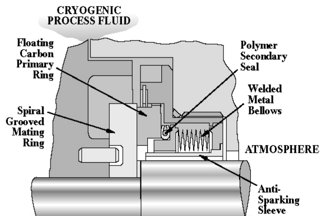
Figure 35. Noncontacting Gas Lubricated Seal for Nonfigure Hazardous Liquefied Gases.
