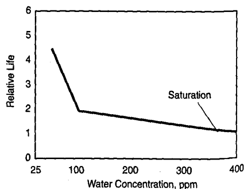
Figure 24. Relative Bearing Life Versus Water Concentration.
