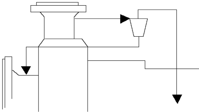
Figure 7. API Plan 31—Use of a Cyclone Separator.
