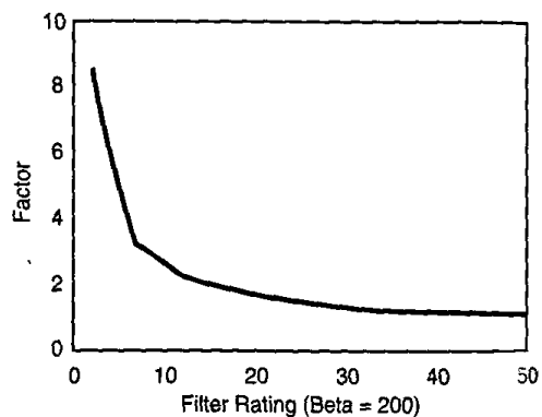
Figure 23. Bearing Life Factor Versus Filter Rating.
