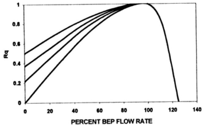
Figure 32. Flow Rate Reliability Factor.
