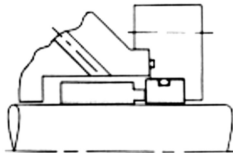
Figure 27. Small Cross-Section ANSI Seal Chamber.
