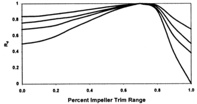
Figure 31. Impeller Diameter Factor.
