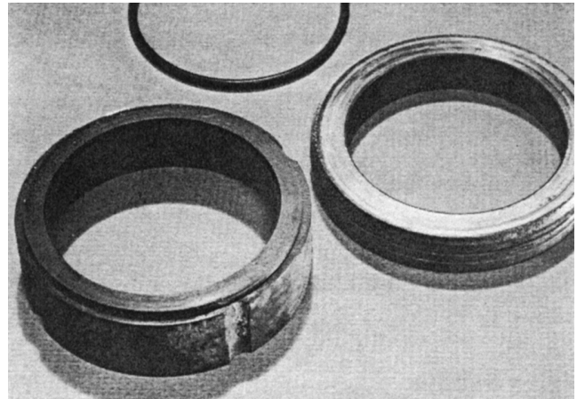
Figure 17. Seal Faces Operated Successfully for 25 Years.
