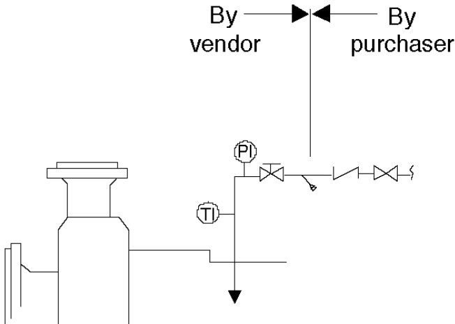
Figure 9. API Plan 32—Clean Fluid Injection from an External Source.
