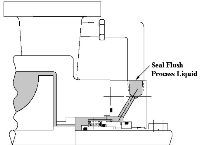
Figure 5. Typical Mechanical Seal Design.
