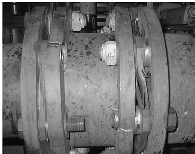
Figure 25. Stress Crack in a Coupling from Misalignment.
