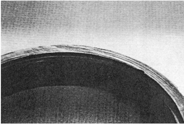
Figure 15. Erosion Damage of a Seal Face.
