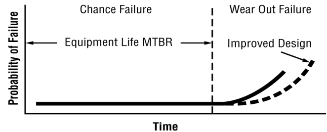
Figure 3. Modified Shape of the Bathtub Curve, Chance and Wear-Out Failures Approach Zero.
