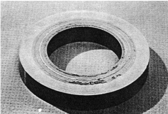
Figure 16. Damage to a Seal Face from Corrosive Wear.
