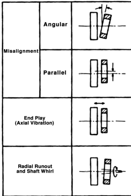
Figure 10. Common Types of Motion Transmitted to a Seal.
