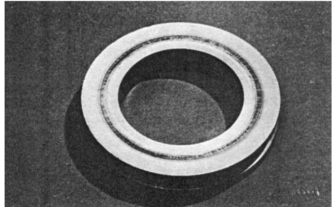
Figure 13. Heat Checking of a Seal Face.
