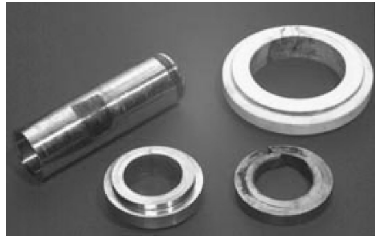
Figure 12. Damage to a Seal from Parallel Misalignment.
