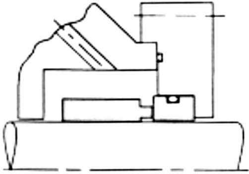
Figure 28. Large Bore ANSI Seal Chamber.
