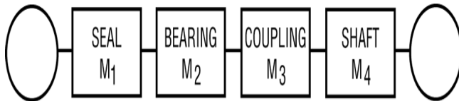
Figure 4. A Series System for an ANSI Pump.
