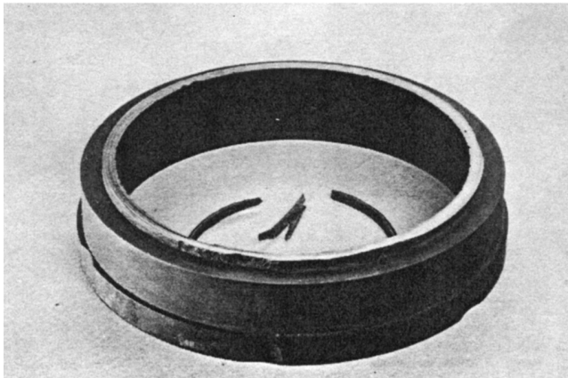
Figure 11. Damage to a Seal from Angular Misalignment.
