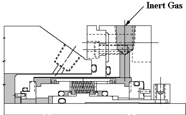
Figure 34. Noncontacting Gas Lubricated Seal Design.
