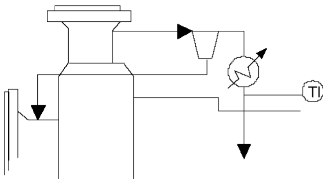
Figure 8. API Plan 41—Use of a Cyclone Separator on Hot Fluids.
