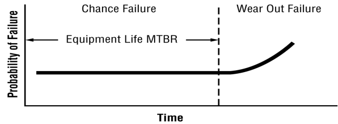
Figure 2. Modified Shape of the Bathtub Curve, Infant Mortality Phase Eliminated.
