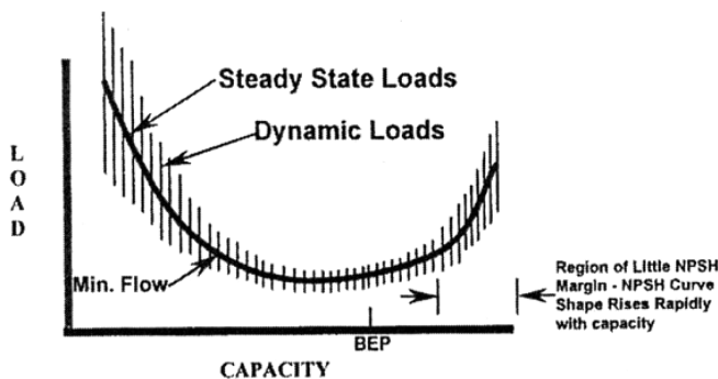
Figure 21. Pump Load-Capacity Curve.
