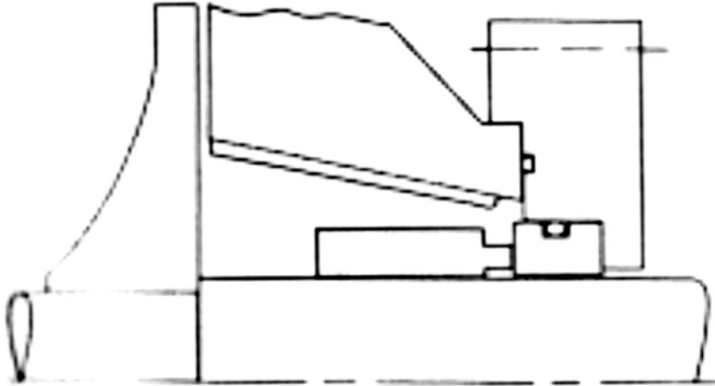
Figure 29. Taper Bore ANSI Seal Chamber.
