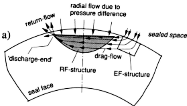
Figure 33. Laser Face Seal Geometry.
