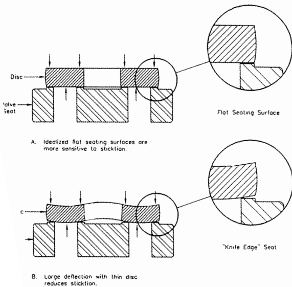
Imperfect Valve Seating Due to Disc Flexibility.
