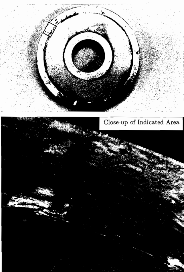
Figure 2. Typical Stricktion Induced Valve Disc Damage.
