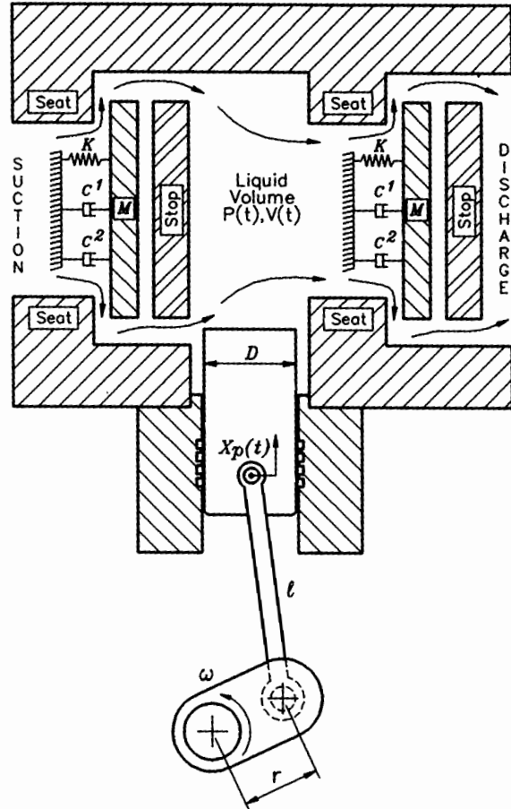
Figure 6. Pump Cylinder Valve Model Parameters.
