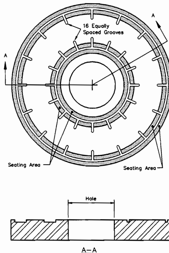
Figure 4. Groove Pattern to Reduce Sticktion.
