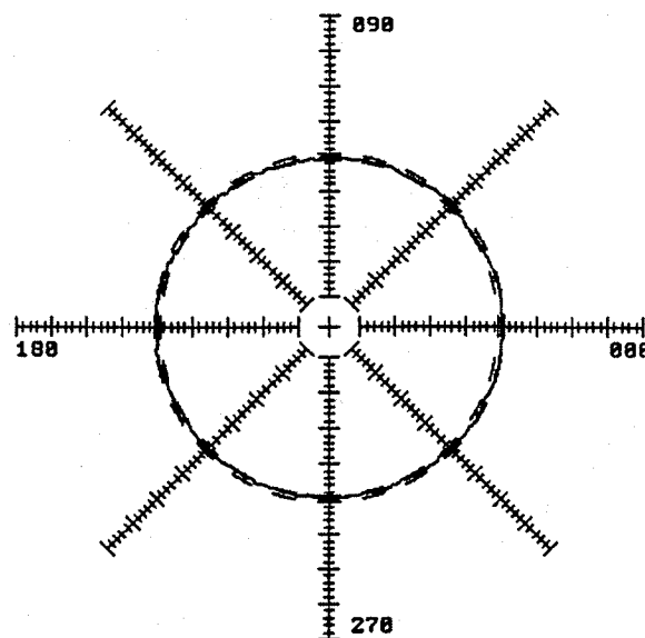
Figure 6. Mating Ring Flatness Measurement.
