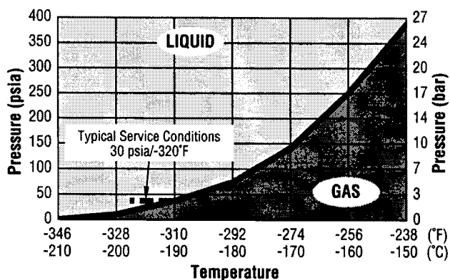
Figure 4. Vapor Pressure Curve for Nitrogen.
