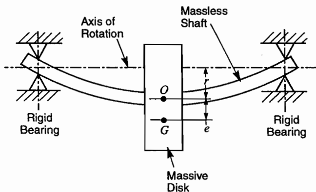
Figure 1. Jeffcott Rotor.
