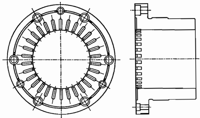
Figure 18. Swirl Brake.
