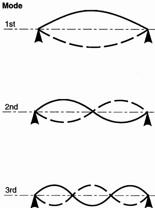
Figure 8. Typical Mode Shapes in Rigid Bearing Regime.
