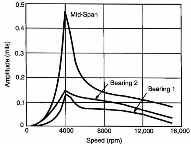
Figure 11. Representative Unbalance Response Plot.
