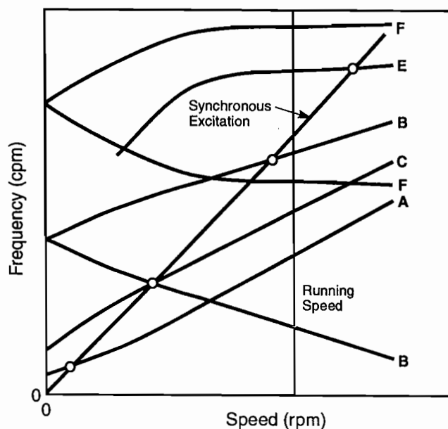
Figure 13. Typical Unabridged Campbell Diagram.
