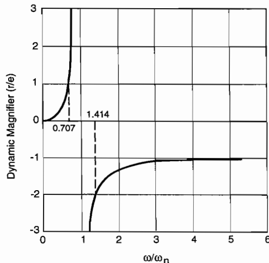
Figure 2. Undamped Response of Jeffcott Rotor.
