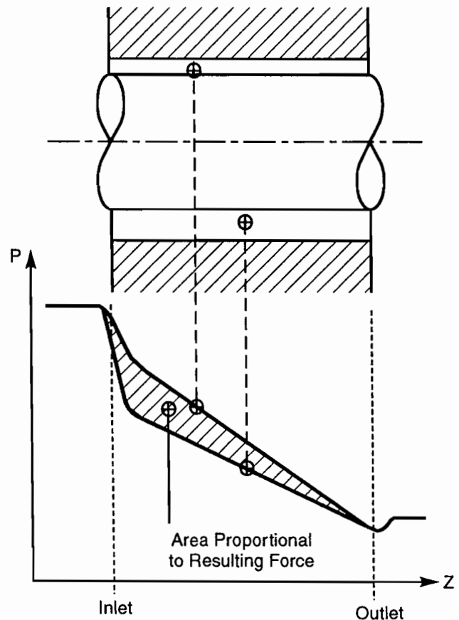
Figure 15. Annular Seal Axial Pressure Distribution.
