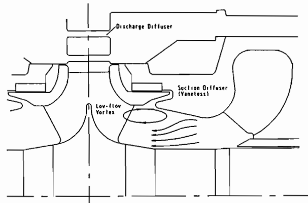
Figure 3. Double-entry Impeller with Suction Diffuser and Discharge Diffuser.
