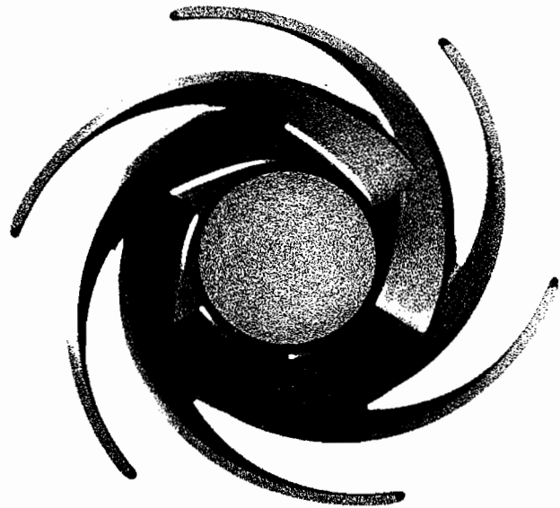
Figure 17. Vanes and Transition Zones towards the Hub Modelled by Splines; Lateral View of a Double-Entry Impeller without Front Shroud.
