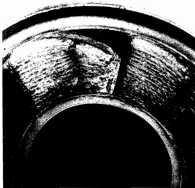
Figure 6. Impeller Vanes Immediately after Surfacing by Welding.
