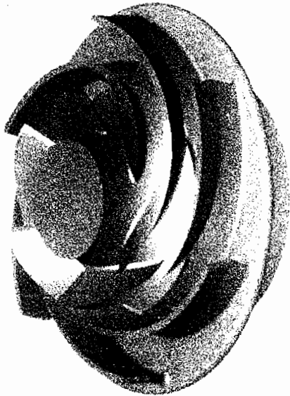
Figure 18. Vanes and Transition Zones towards the Hub and Front Shroud Modelled by Splines. For a better presentation of the vane curvature of the profiled vanes, one of the front shrouds has been omitted.
