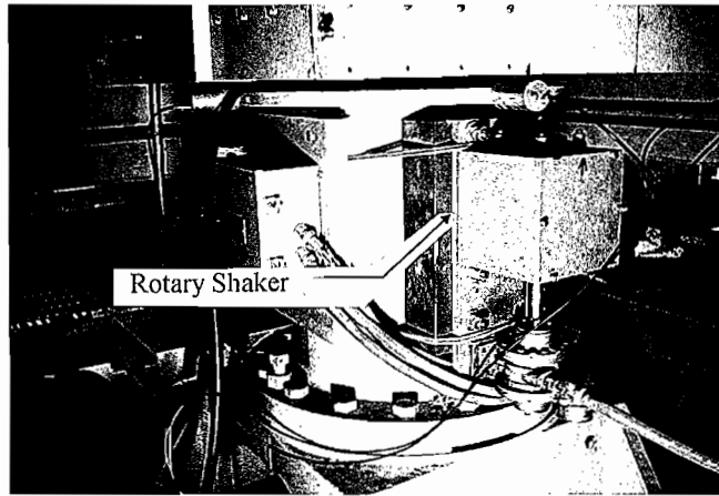
Figure 29. Shaker Installed on Pump Housing.
