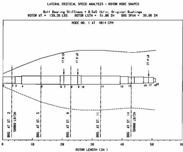
Figure 11. Pump Rotor Model and Vibration Mode Shape.
