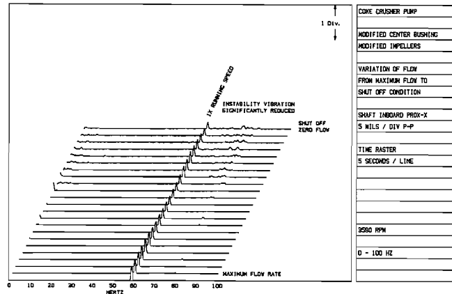
Figure 18. Frequency Spectra of Shaft Vibration (Modified Center Bushing) vs Pump Operating Conditions.
