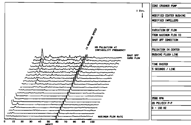
Figure 19. Frequency Spectra of Pulsation in Center Bushing Flush Line with Modified Center Bushing.
