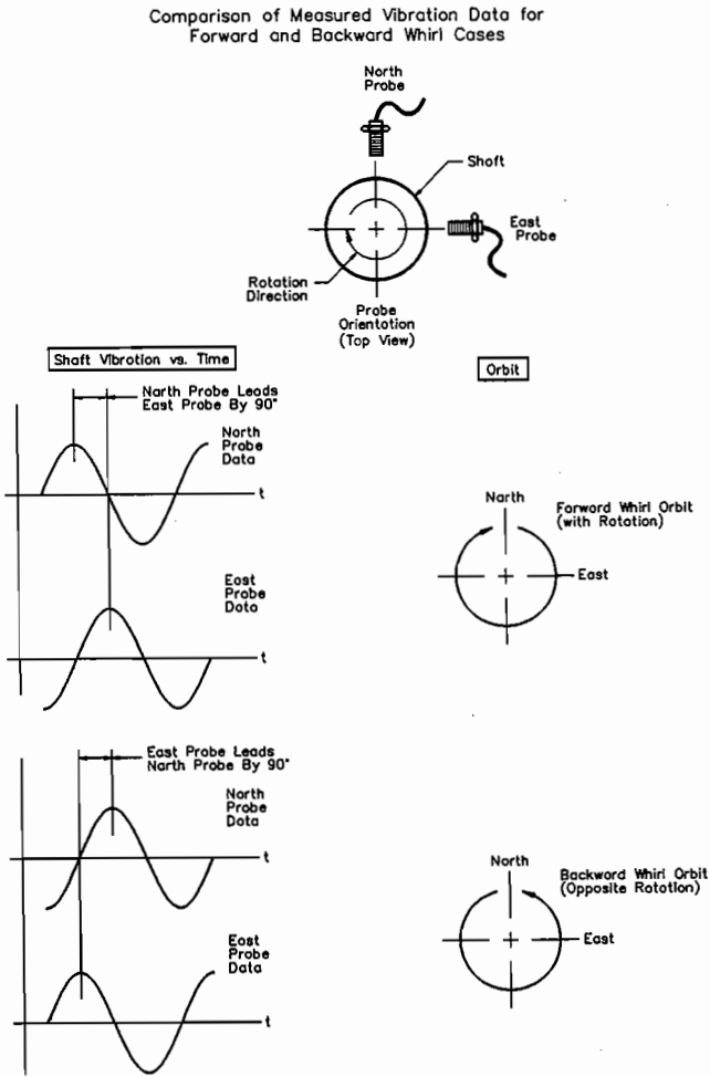
Figure 24. Comparison of Measured Vibration Data for Forward and Backward Whirl Cases.
