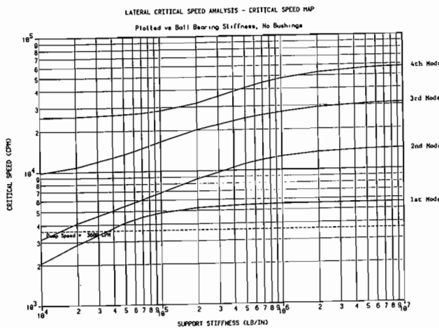
Figure 12. Lateral Critical Speed Map.
