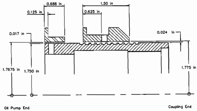
Figure 16. Original Throat Bushing-Oil Pump End (Grooved Stator).
