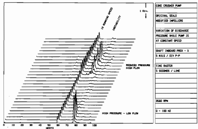
Figure 8. Frequency Spectra of Shaft Vibration vs Pump Discharge Pressure.
