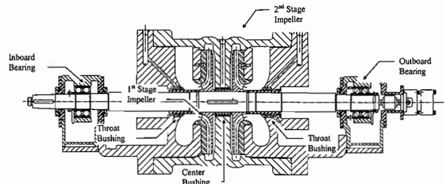
Figure 3. Pump Cross Section.
