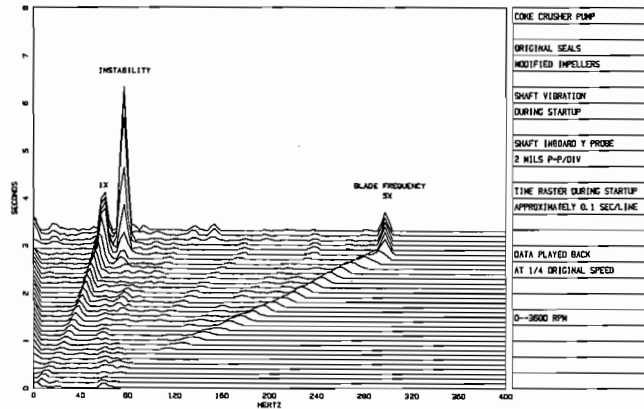
Figure 5. Shaft Instability Vibration During Startup—Original Bushings.
