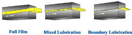
Figure 9. Three phases of lubrication film
