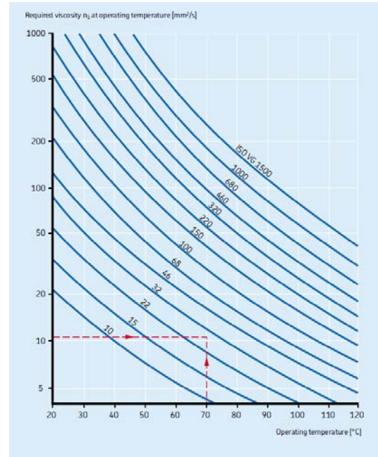
Figure 8. Oil viscosity at operating temperature for standard mineral oils
