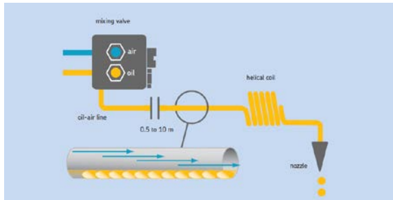
Figure 13. Oil/Air lubrication introduces very small amounts of oil into the bearings
