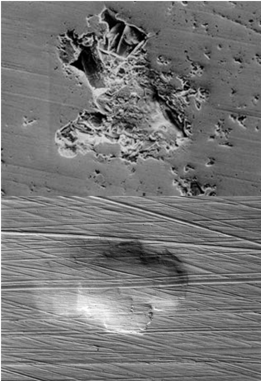
Figure 3. Hard particle dent (top) and a soft particle dent (bottom) can both be damaging
