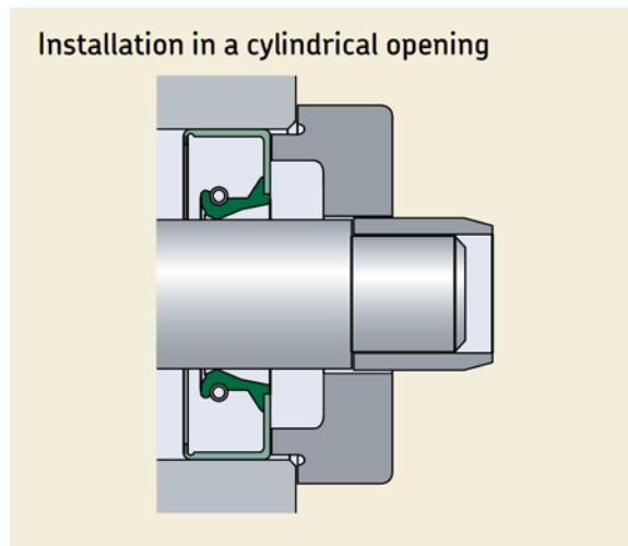
Figure 4. Proper installation of a seal including use of shaft sleeve and fitting tool
