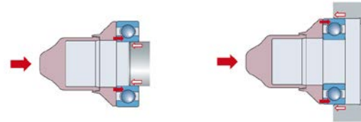
Figure 15. A sleeve should be used when pressing a bearing onto a shaft or into a housing
