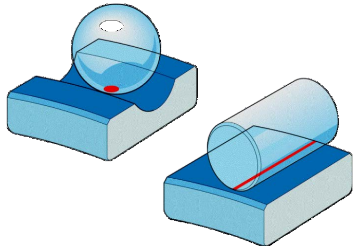
Figure 2. Contact areas for ball and roller bearings endure very high pressures.
