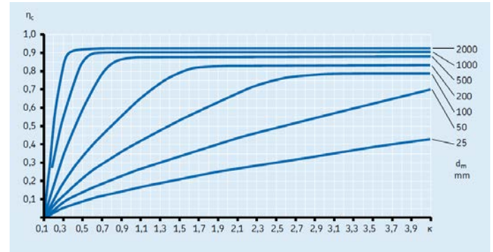
Figure 10. Contamination factor for circulating oil with solid contaminant level 18/15/12, ISO 4406
