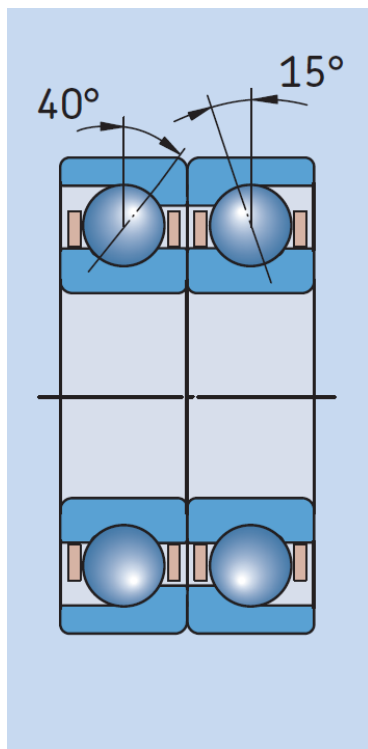
Figure 19. Angular contact bearing pair with dissimilar contact angles
