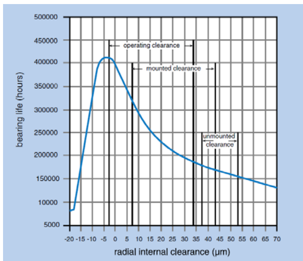
Figure 18. Operating clearance is a function of shaft fit and thermal effects
