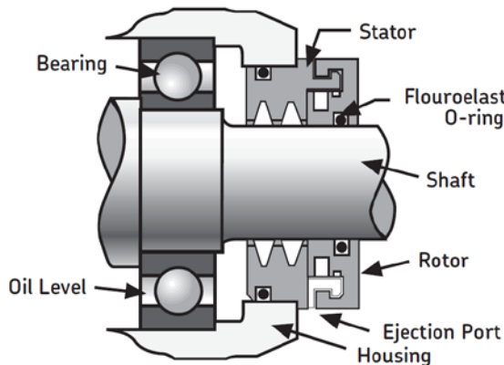
Figure 6. Isolator type labyrinth seal
