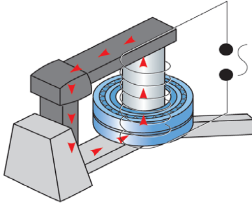
Figure 16. Induction heaters rapidly heat the bearing by creating current in the bearing rings
