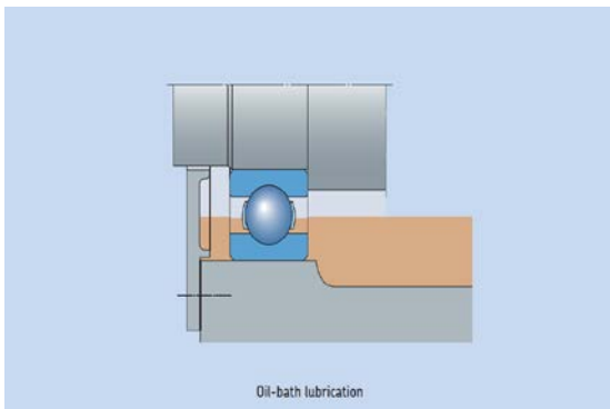
Figure 11. Typical oil bath arrangement and bath height for a deep groove ball bearing
