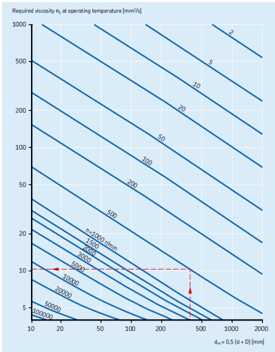
Figure 7. Required viscosity in centistokes ( \text{mm}^2/\text{s} ) as a function of shaft speed and bearing size
