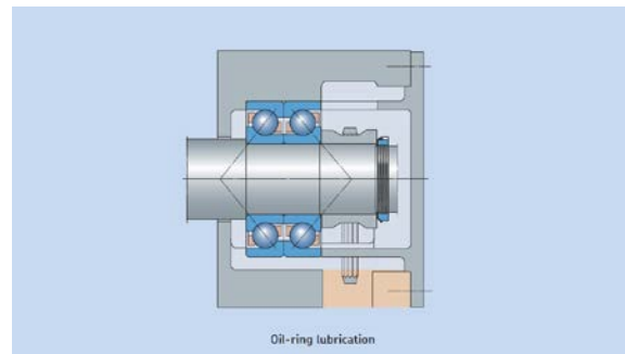
Figure 12. Typical oil ring system with the oil sump well below the bearing.
