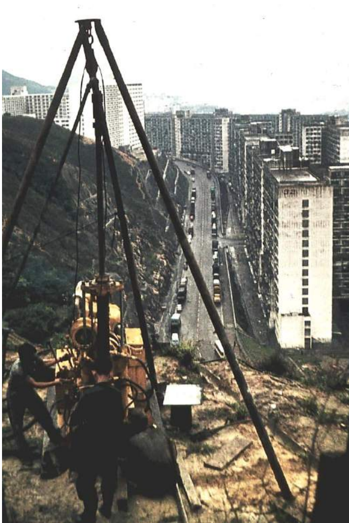
Figure 11: Drilling vertical diamond core holes into the Sau Mau Ping slope. These holes were used for geotechnical investigation purposes and also for the installation of piezometers in the rock mass.
