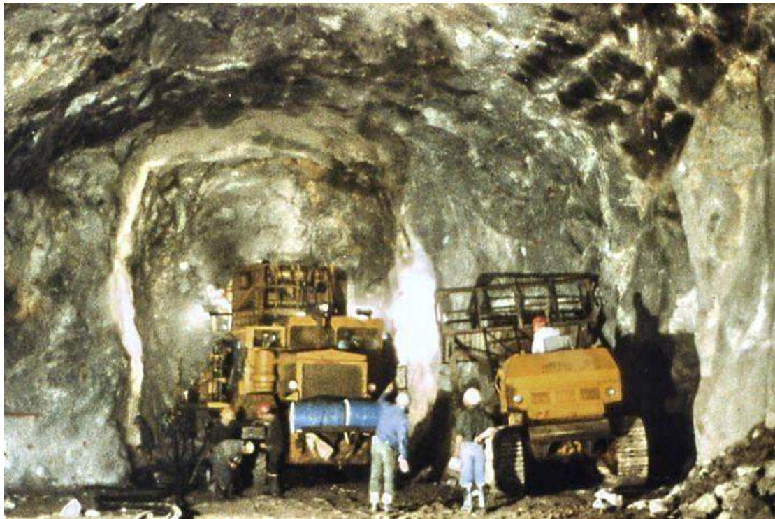
Figure 4: A 6 m wide heading driven ahead of the tunnel face to permit pre-reinforcement of potentially unstable wedges in the roof. The seven-boom jumbo is seen working in the heading.
