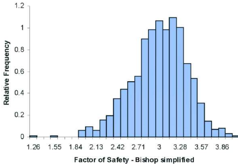
Figure 15: Distribution of factors of safety for the slope shown in Figure 14 from a probabilistic analysis using the program SLIDE.
