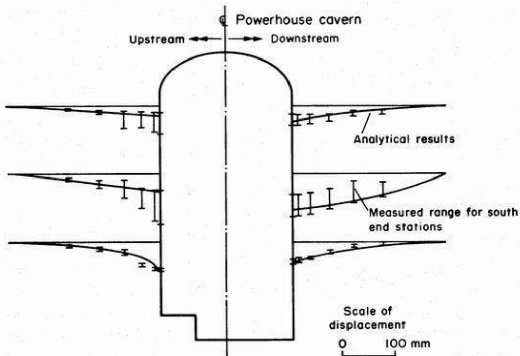
Figure 23: Comparison between predicted and measured deformations in the Mingtan power cavern sidewalls.
