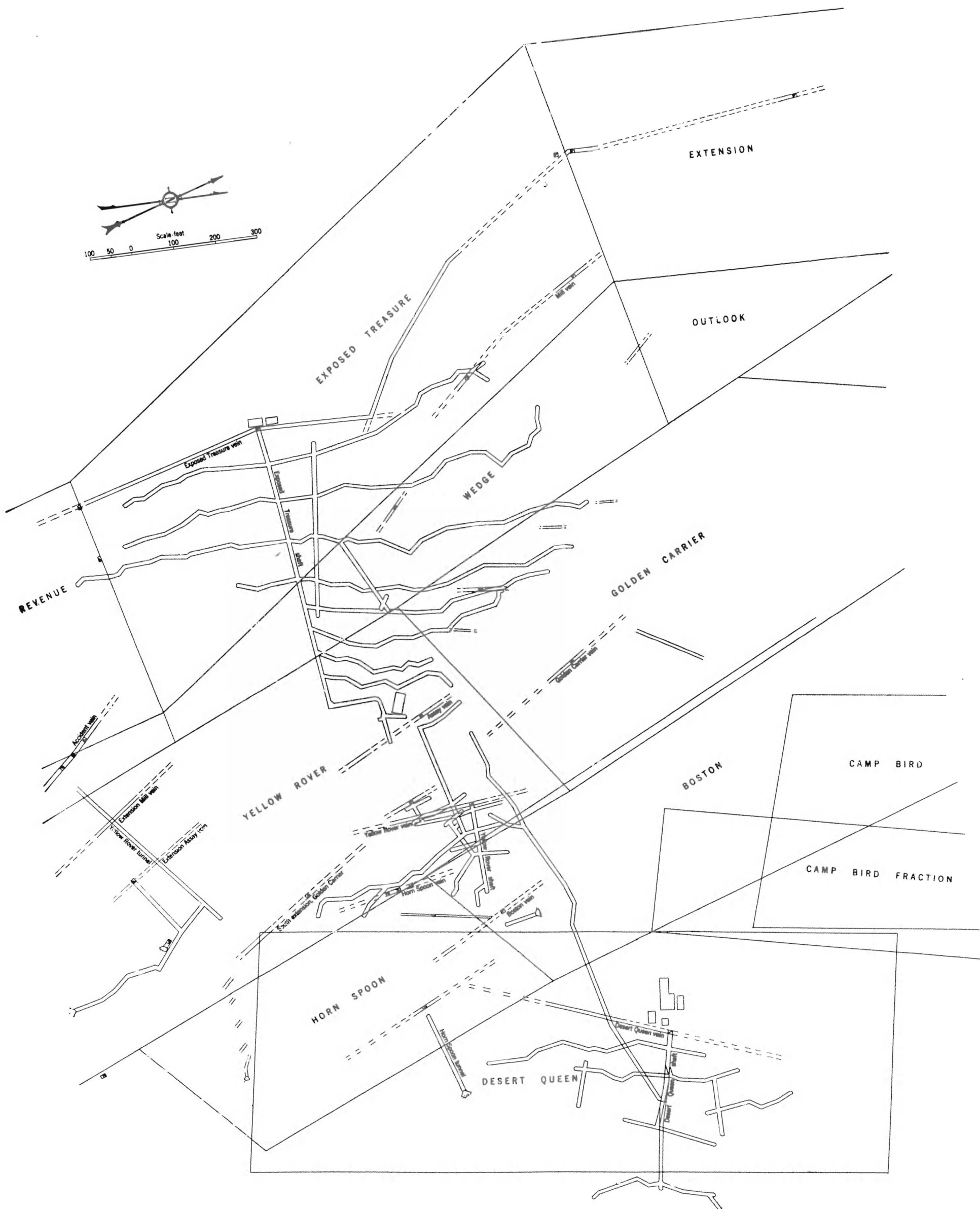
FIGURE 9.- Plan of Exposed Treasure, Yellow Rover and Desert Queen mines.
