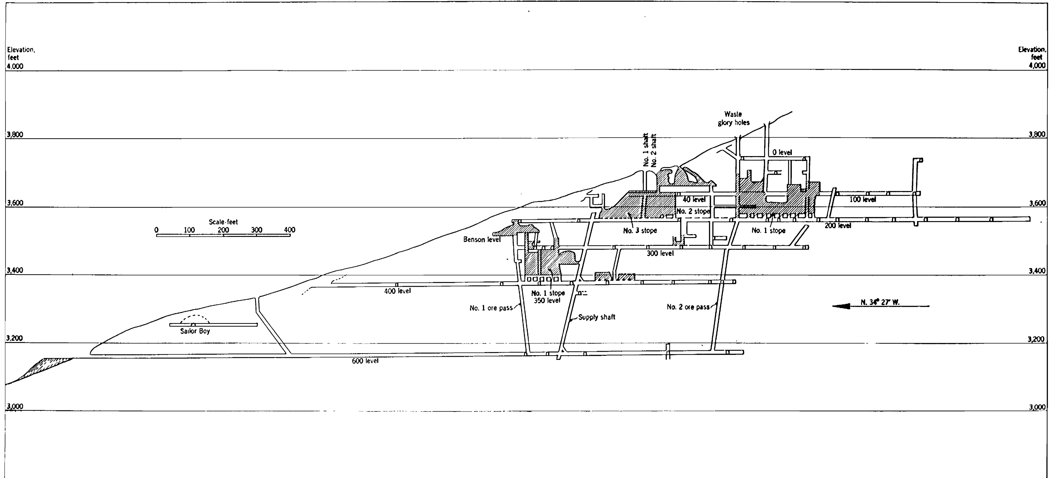
FIGURE 6. Longitudinal projection of Golden Queen mine.
