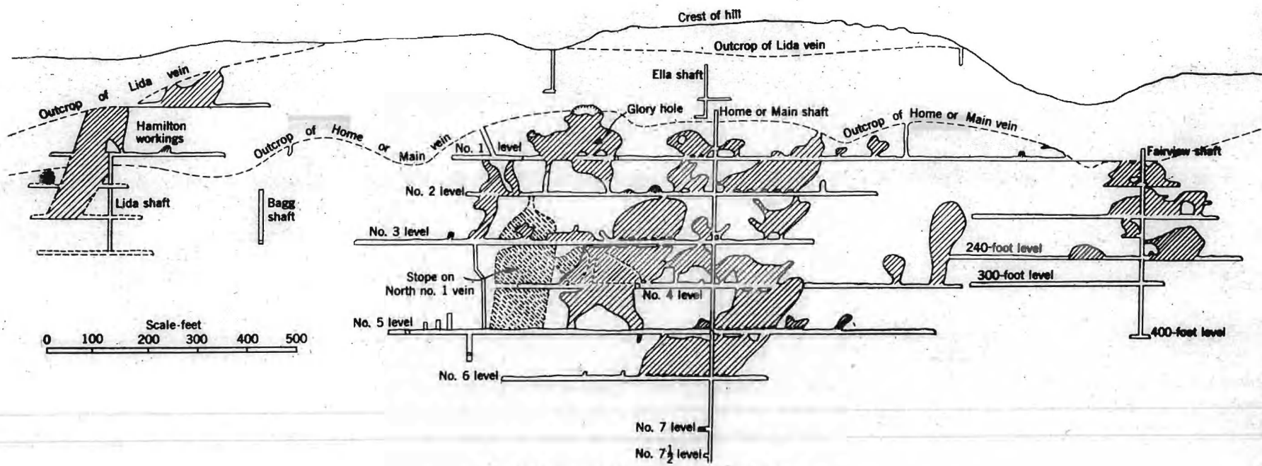
FIGURE 10.- Longitudinal projection of Tropico mine.
