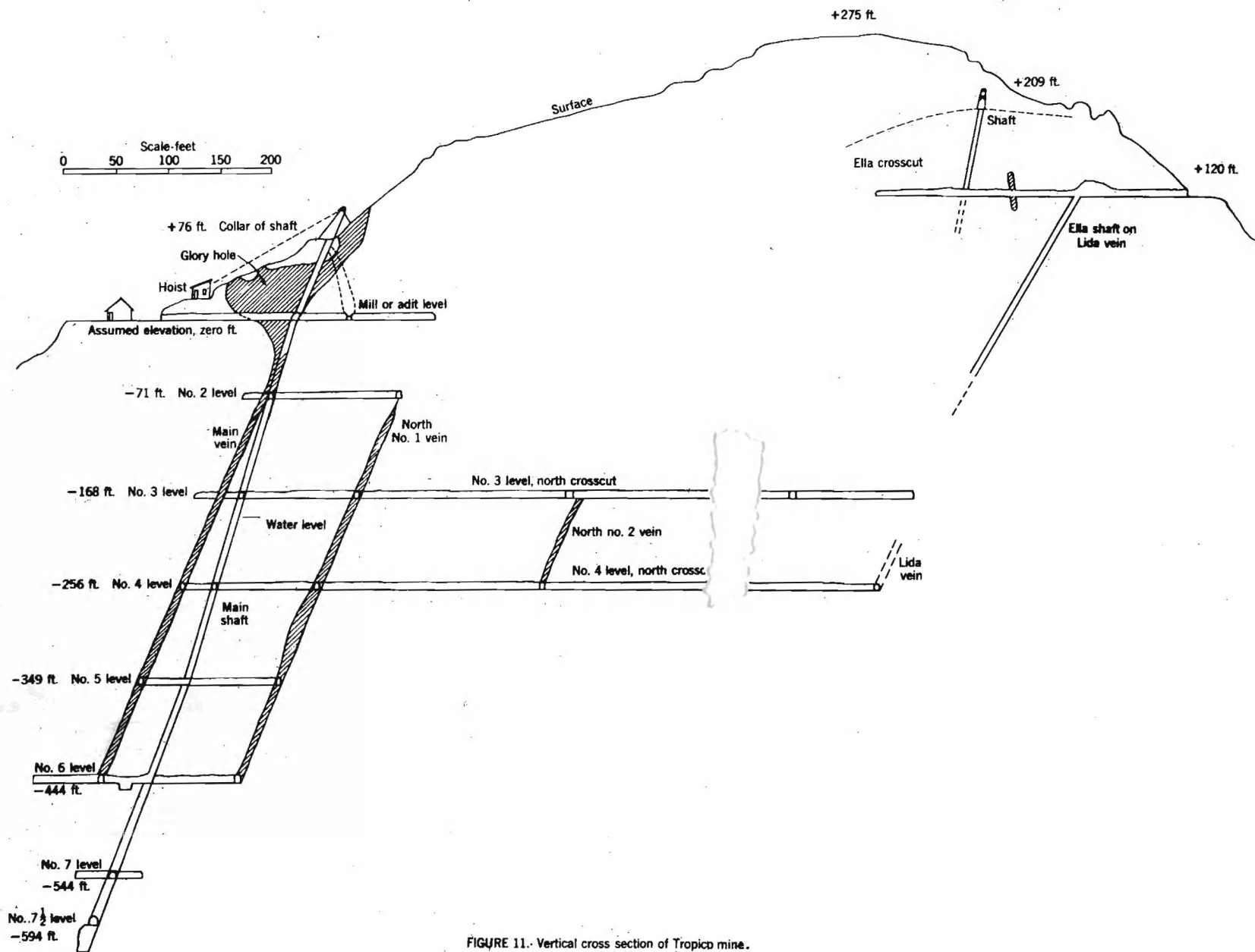
FIGURE 11. Vertical cross section of Tropic mine.
