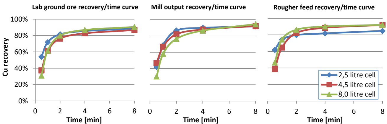
Figure 5.1: Cu recovery as a function of time for batch tests on different materials.
