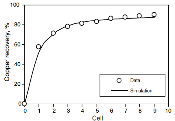
Figure 3.9: Plant survey recovery results and model prediction (Yianatos et al., 2005b).
