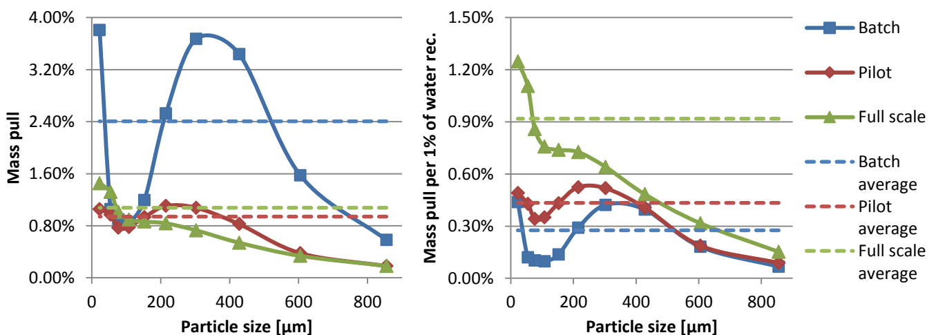
Figure 5.38: Mass pull (left) and mass pull normalized per 1% water recovery (right) vs. particle size.
