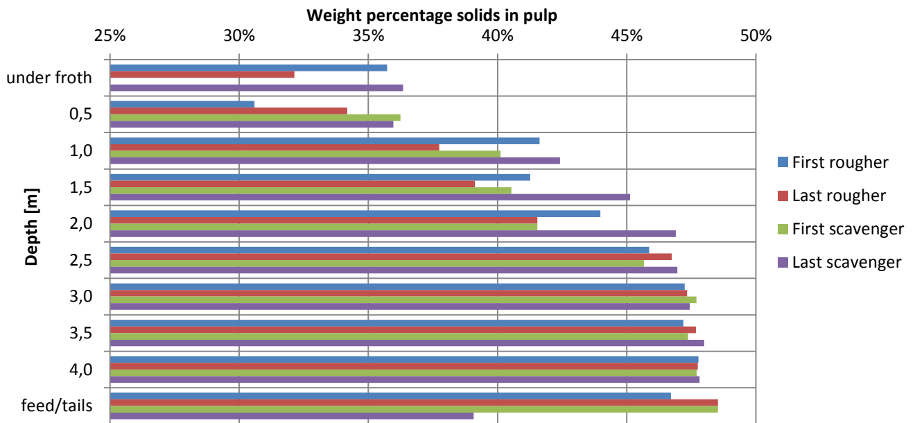
Figure 5.15: Weight percentage solids in pulp per cell for Aitik survey on 04-11-2013.
