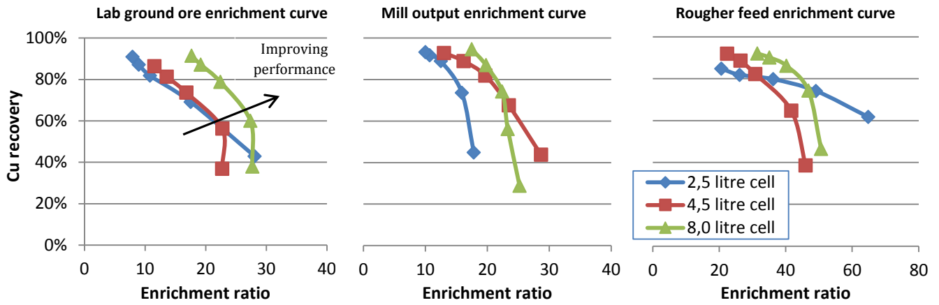
Figure 5.4: Cu recovery vs. enrichment ratio for batch tests on different materials.
