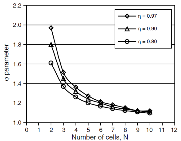
Figure 3.10: Mixing parameter \varphi versus the number of cells in a bank, at different dimensionless recoveries (Yianatos, 2005b).
