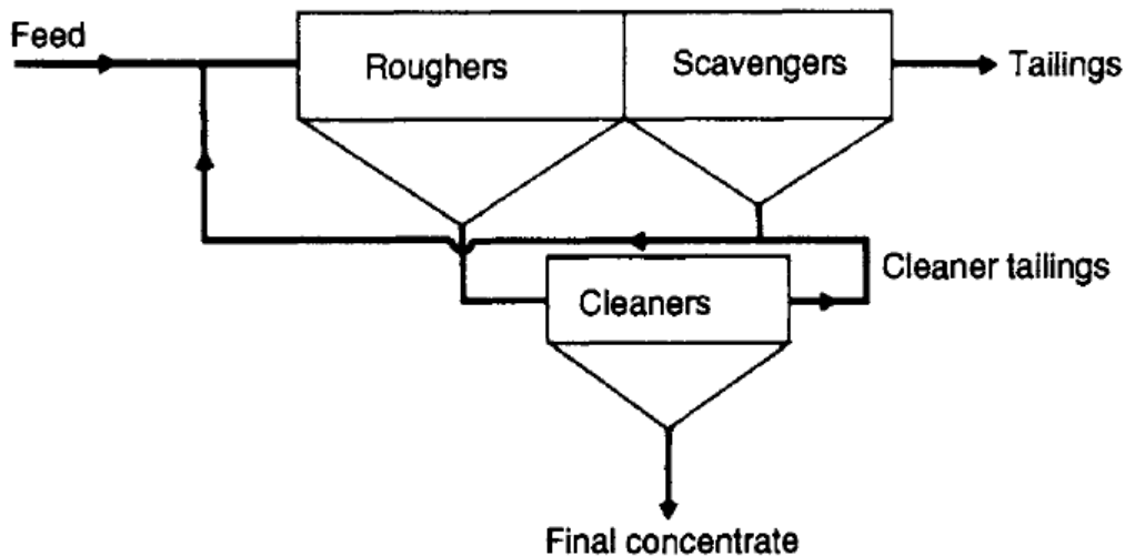
Figure 2.1: Example of a basic flotation system with roughers, scavengers and cleaners (Wills, 2006).
