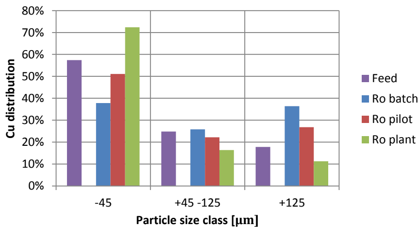
Figure 5.30: Copper distribution in feed and tailings over the different size classes in rougher flotation.
