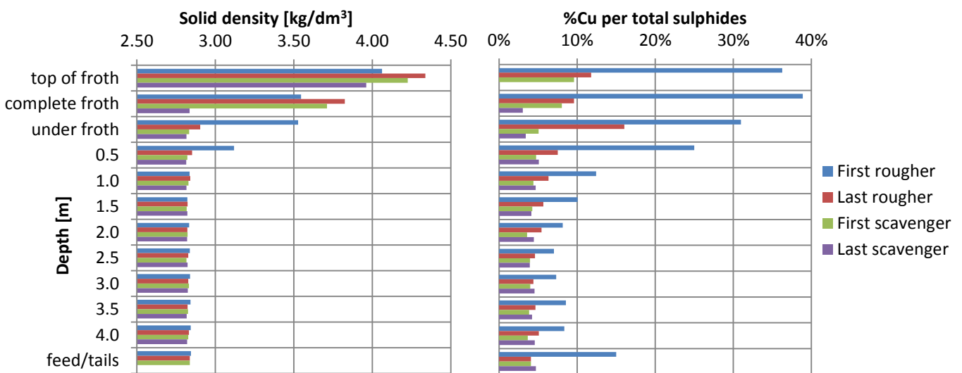
Figure 5.19: Solid density and Cu-percentage in sulphides per cell for Aitik survey on 04-11-2013.
