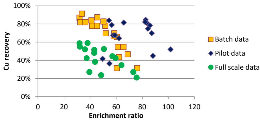
Figure 5.33: Copper recovery vs. enrichment ratio in rougher flotation.
