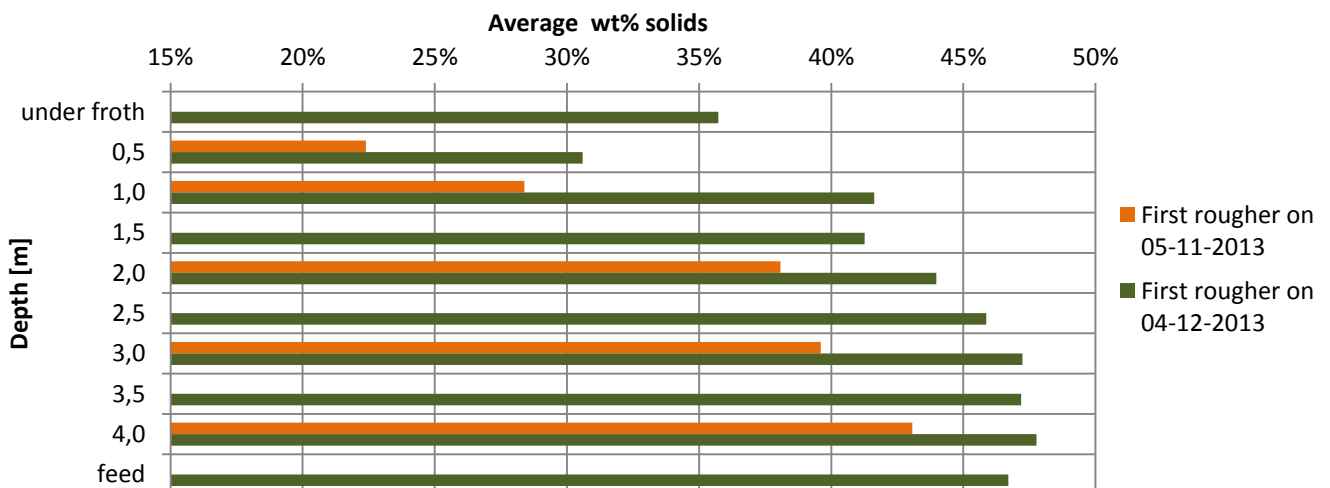
Figure 5.16: Average weight percentage solids in pulp per cell for Aitik survey on 04-11-2013.
