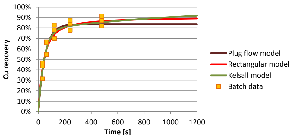
Figure 5.28: Rougher batch test results modelled according to three different methods.
