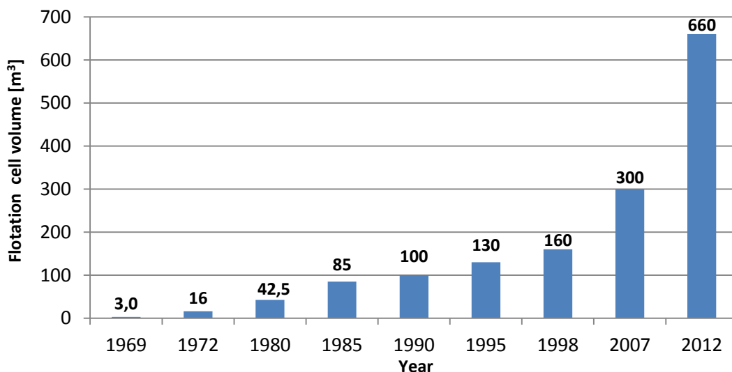
Figure 1.2: Largest available mechanical flotation cell volumes on the market since 1972. (Arbiter, 2000; Govender et al., 2014).
