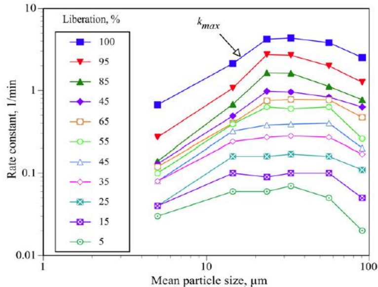
Figure 2.2: Flotation rate constants as a function of particle size for different liberation classes (Jameson, 2012).
