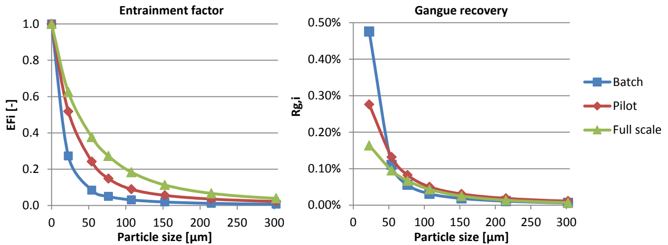
Figure 5.37: Entrainment factor (left) and corresponding gangue mineral recovery (right) versus particle size.
