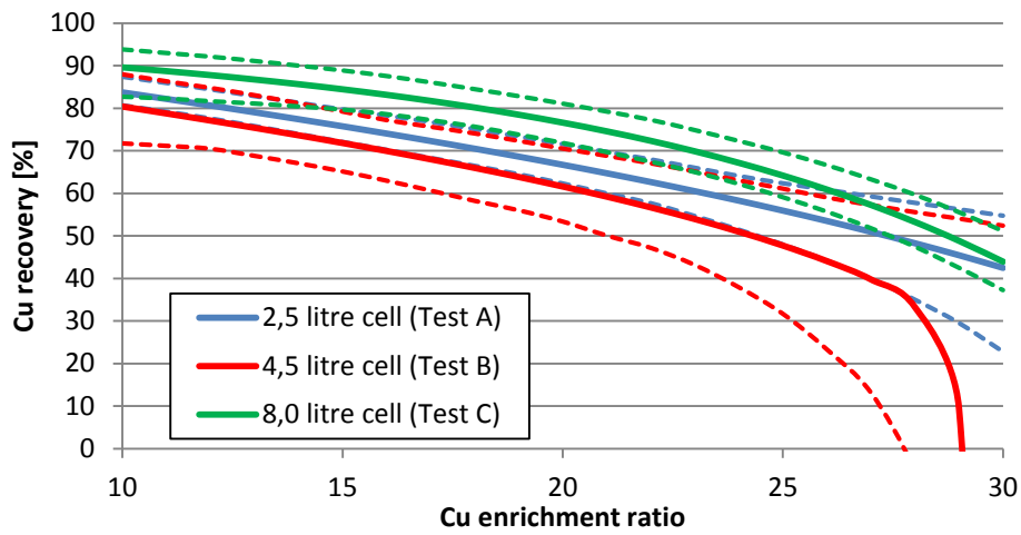
Figure 5.5: Modelled ER-recovery curves of copper with the corresponding upper and lower confidence intervals (dotted lines).
