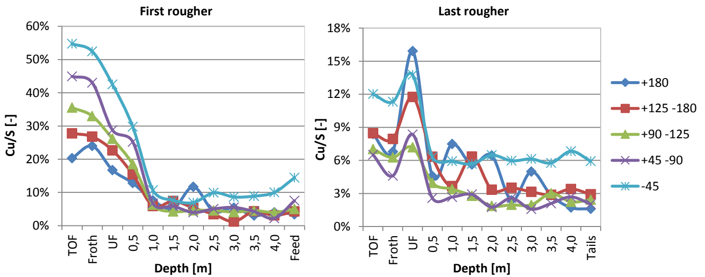
Figure 5.20: Copper content in the total sulphides (Cu/S) vs. cell depth for the first and last rougher cell.
