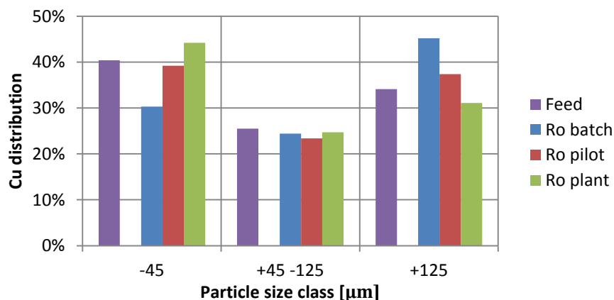
Figure 5.32: Copper distribution in feed and tailings over the different size classes in scavenger flotation.
