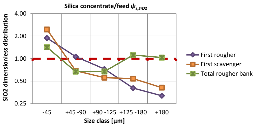
Figure 5.27: Silica dimensionless distribution between feed and concentrate per size class.
