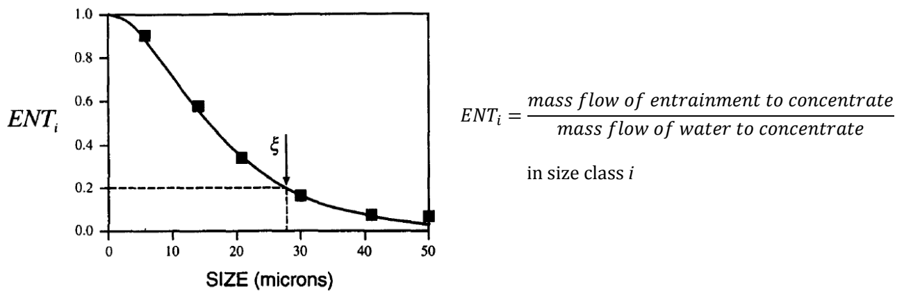
Figure 2.5: Empirical partition curve for entrainment (Savassi et al., 1998).
