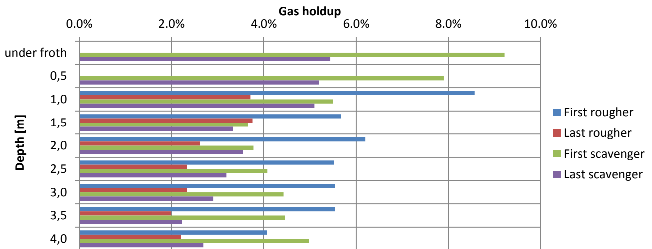
Figure 5.13: Gas holdup per cell for Aitik survey on 04-11-2013. No reliable data for first and last rougher under froth and at 0,5 m depth.
