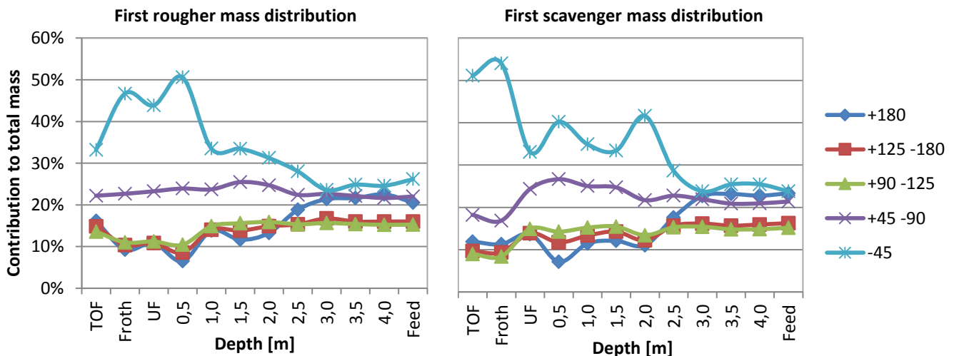
Figure 5.18: Mass distribution curves per size class for the first rougher and first scavenger.
