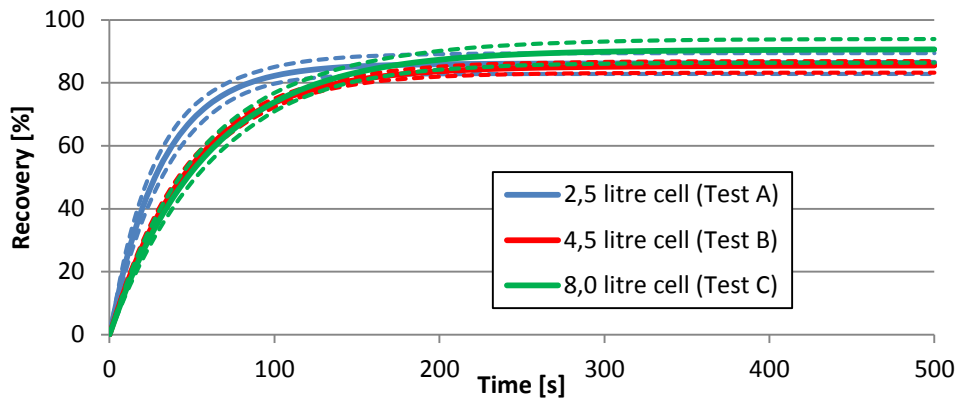
Figure 5.3: Model curves for Aitik crushed ore batch flotation tests with 95% confidence intervals.
