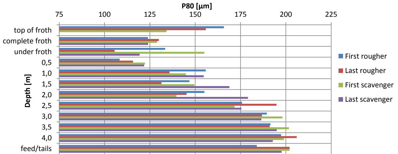
Figure 5.17: P_{80} values per cell as a profile of depth for Aitik survey on 04-11-2013.
