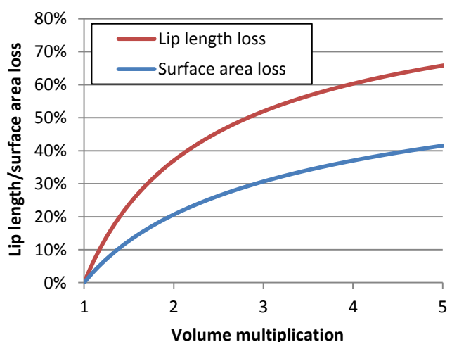
Figure 6.1: Net loss of lip length and surface area during scale-up.
