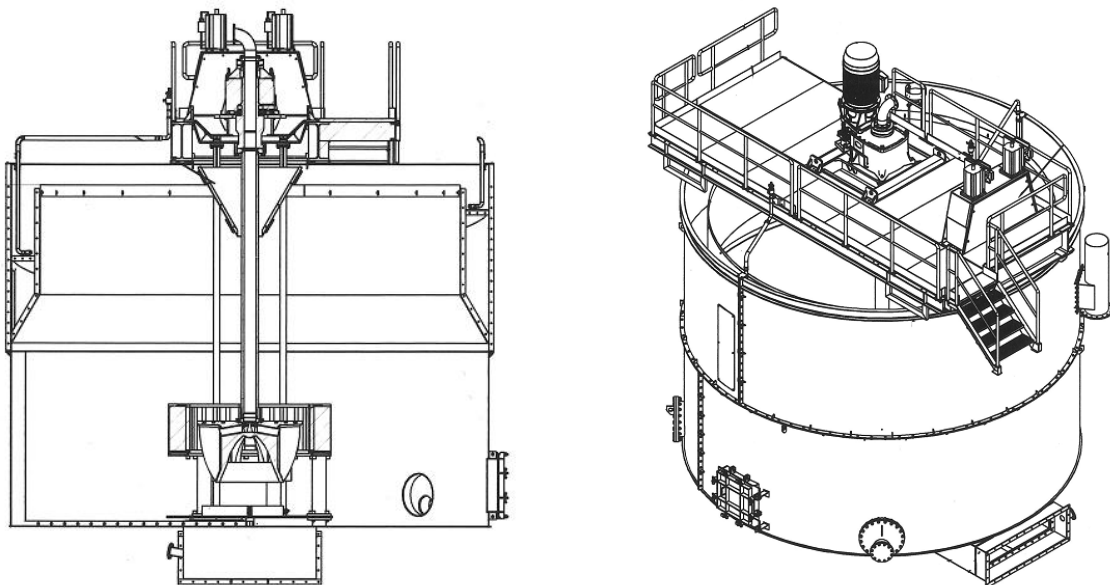
Figure 5.12: Representation of the Outotec TankCell-160 as used by Boliden Aitik (Boliden, 2008).
