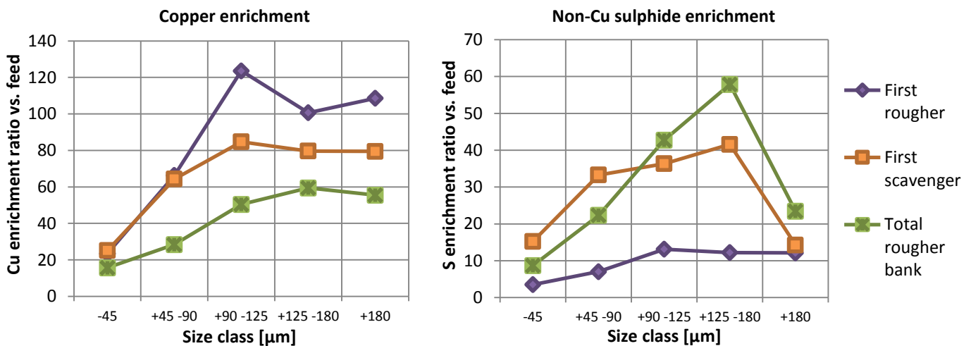
Figure 5.22: Copper and non-Cu sulphide enrichment per size class.
