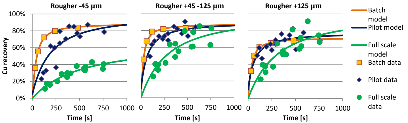
Figure 5.29: Time-recovery test data points and model curves of batch, pilot and full scale rougher tests for three different size classes.
