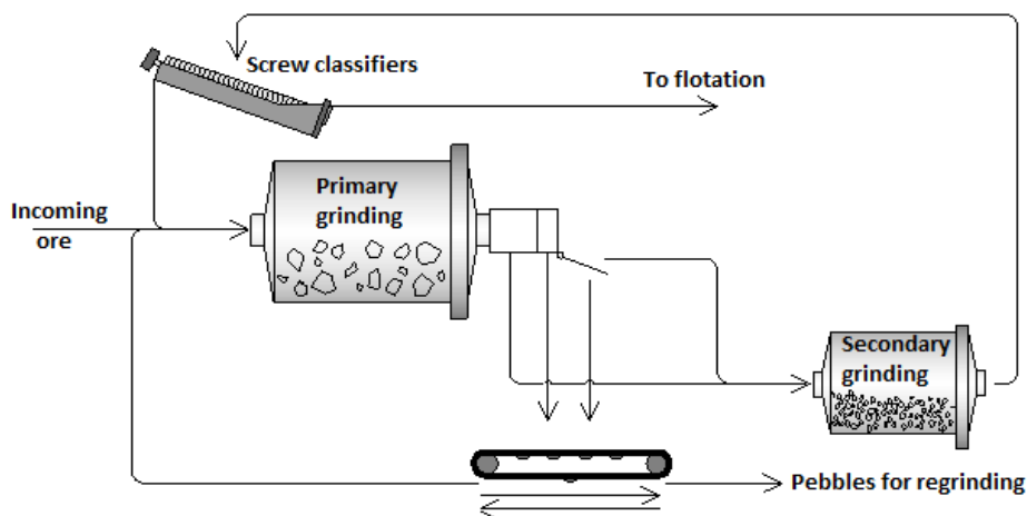
Figure 3.12: Overview of the grinding process at Boliden Aitik.
