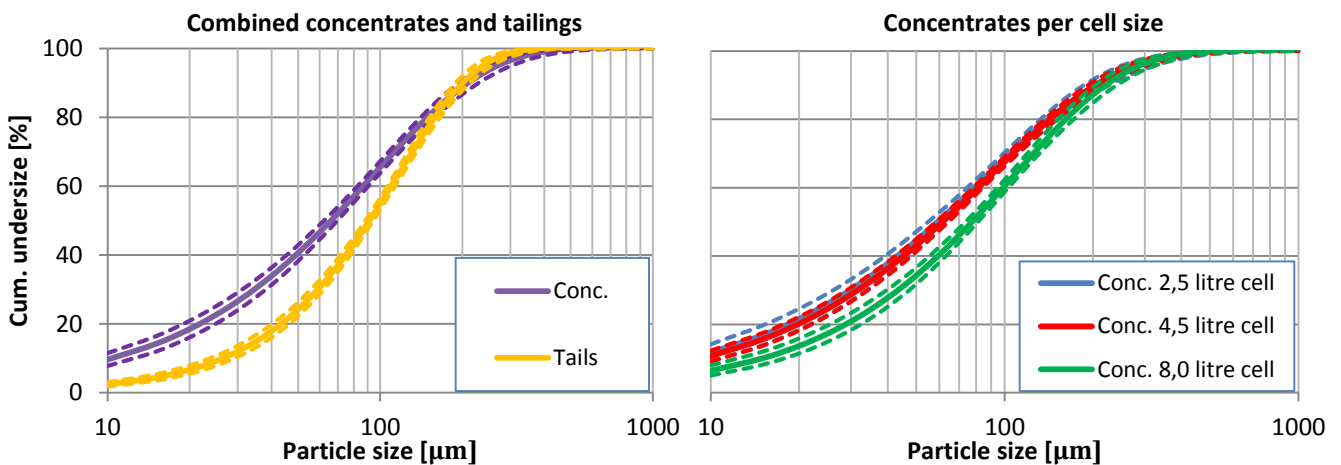
Figure 5.7: Modelled size distribution curves with upper and lower confidence intervals (dotted lines) for batch flotation.
