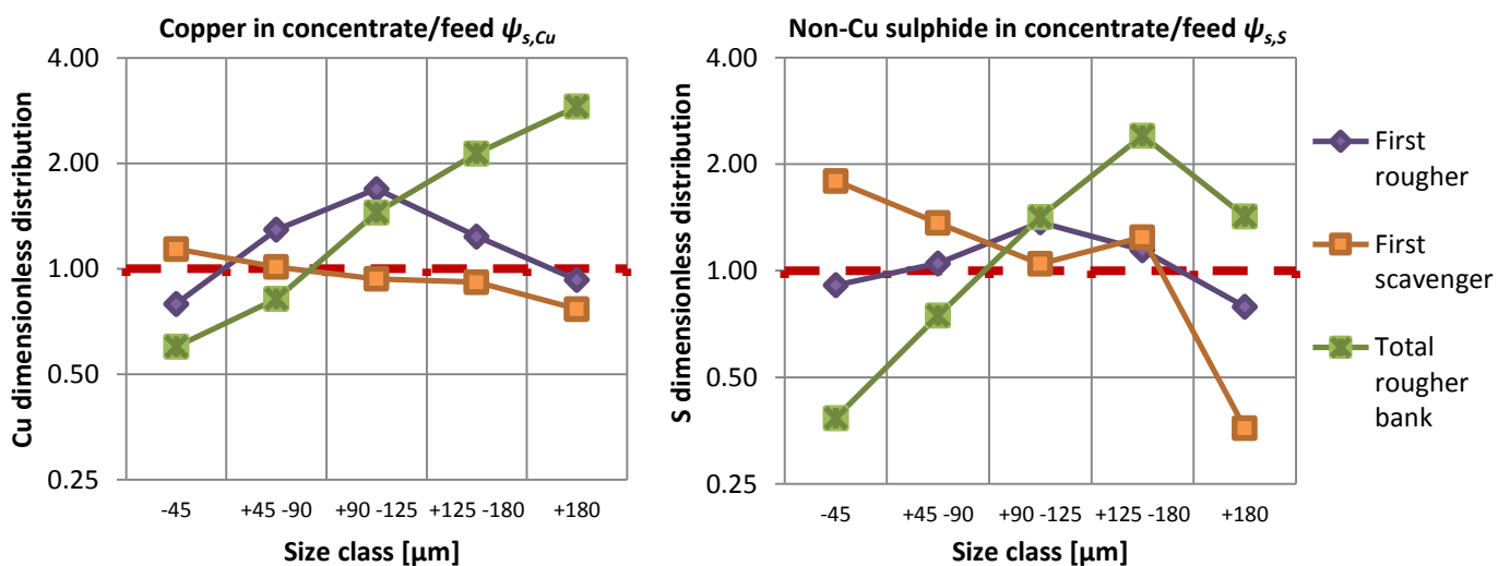
Figure 5.24: Copper and non-Cu sulphide dimensionless distributions of feed vs. concentrate per size class.
