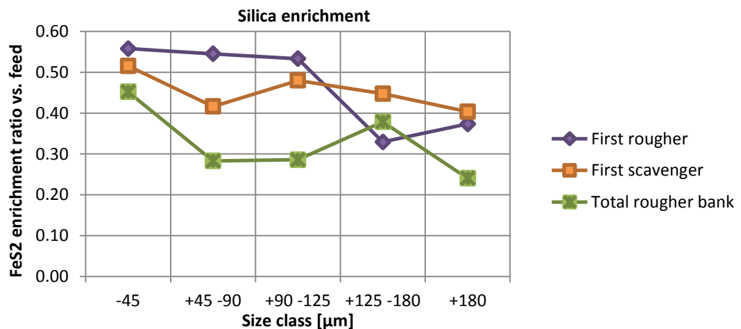
Figure 5.25: Silica enrichment per size class.
