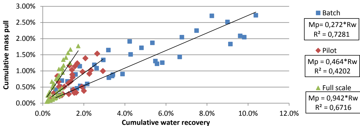
Figure 5.36: Scatter plot with trendlines for the cumulative mass pull vs. the cumulative water recovery.
