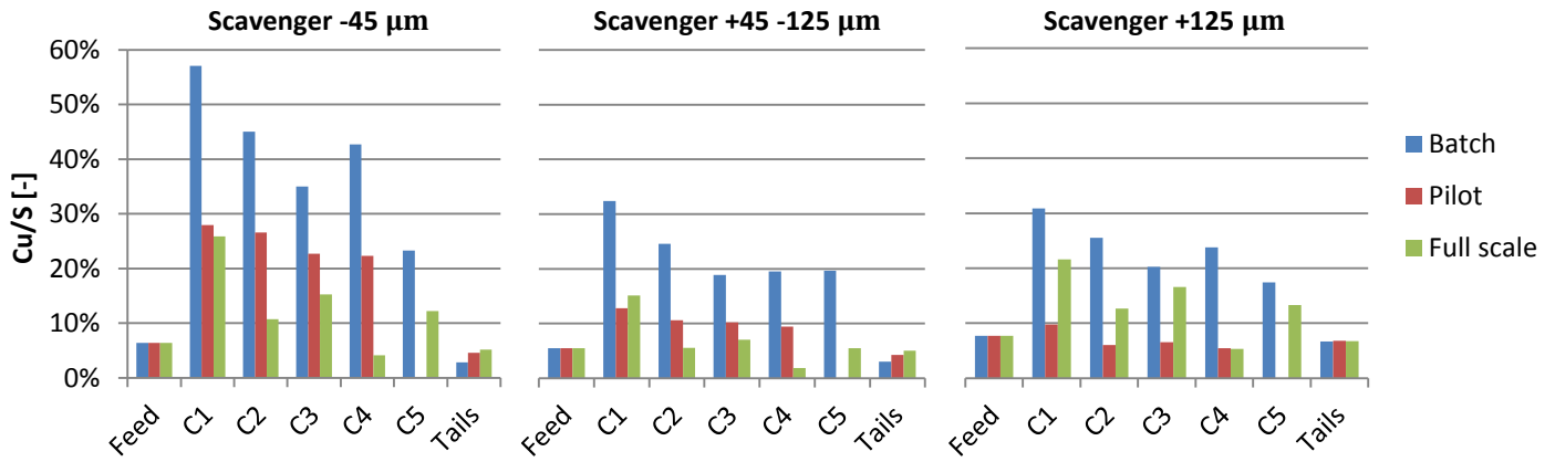
Figure 5.35: Cu/S values for three particle size classes on different scavenger flotation scales.
