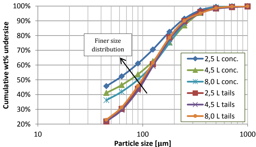
Figure 5.6: Averaged particle size distributions of concentrates and tailings per cell size for batch tests on different materials.
