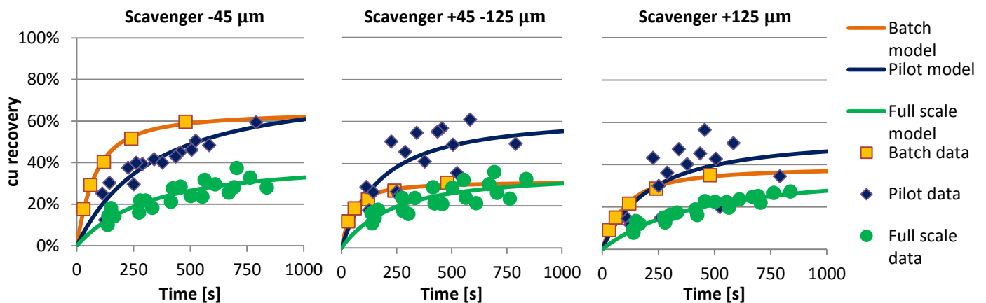
Figure 5.31: Time-recovery test data points and model curves of batch, pilot and full scale scavenger tests for three different size classes.
