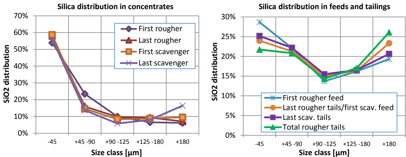
Figure 5.26: Silica distributions in concentrates, feeds and tailings of various cells.
