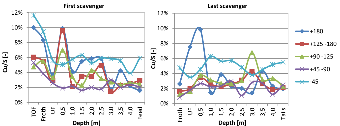
Figure 5.21: Copper content in the total sulphides (Cu/S) vs. cell depth for the first and last scavenger cell.
