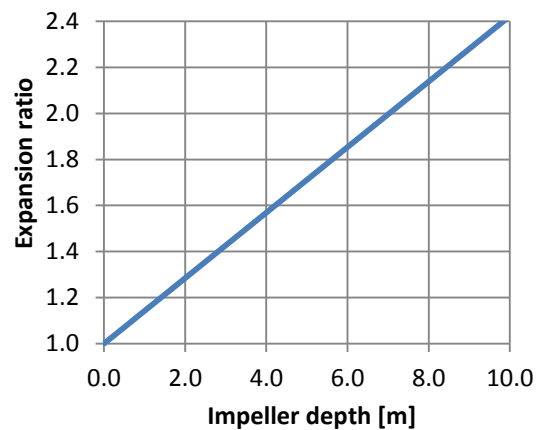
Figure 3.2: Bubble volume expansion ratio as a function of impeller depth.
