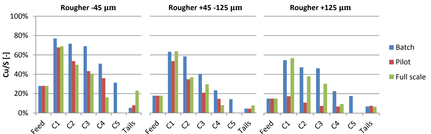
Figure 5.34: Cu/S values for three particle size classes on different rougher flotation scales.
