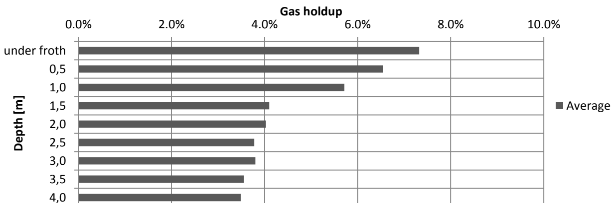
Figure 5.14: Average gas holdup for Aitik survey on 04-11-2013.
