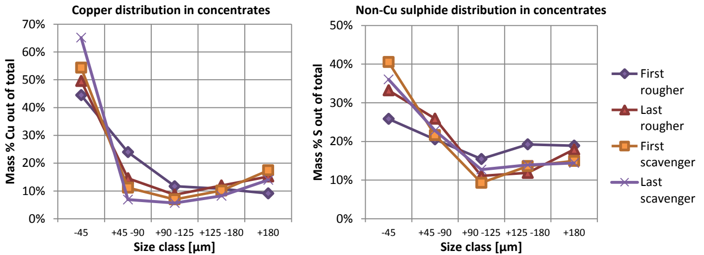
Figure 5.23: Copper and non-Cu sulphide distribution in the concentrates per size class.
