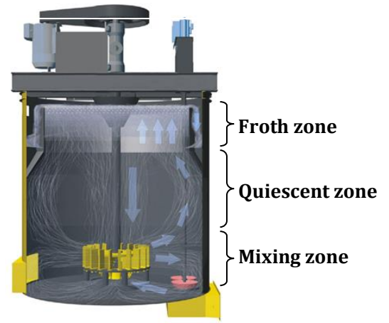
Figure 3.1: Subzones of a flotation cell (Outotec, 2014).
