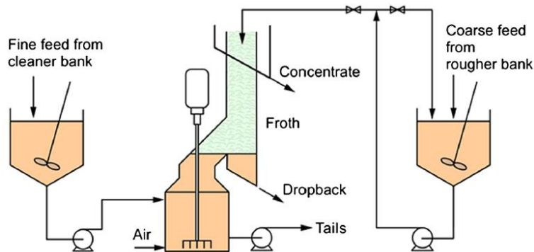
Figure 2.4: Test apparatus used for coarse particle flotation by Ata and Johnson (2013).
