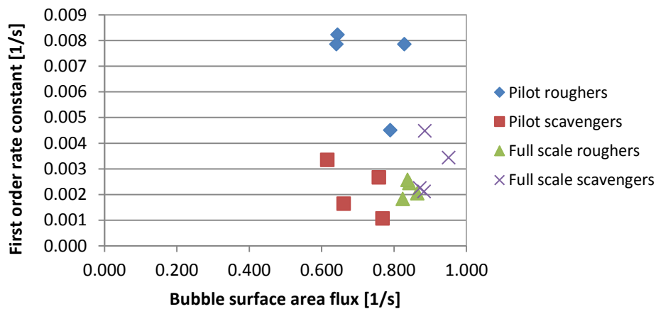
Figure 5.39: Plot of the bubble surface area flux ( S_b ) vs. the first order flotation rate constant ( k ).
