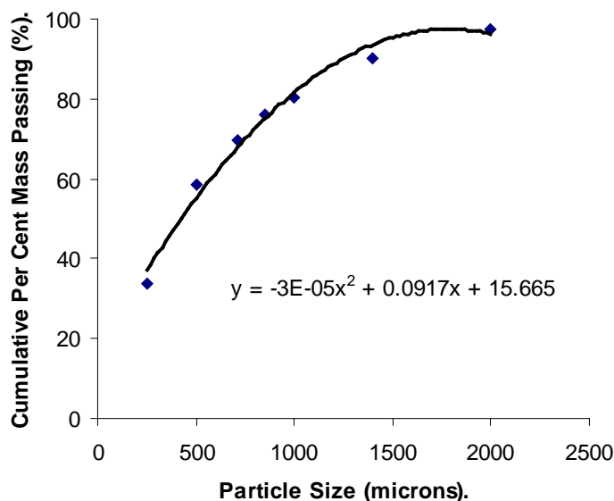
Figure 2: Reference ore (quartz) discharge, particle size analysis
