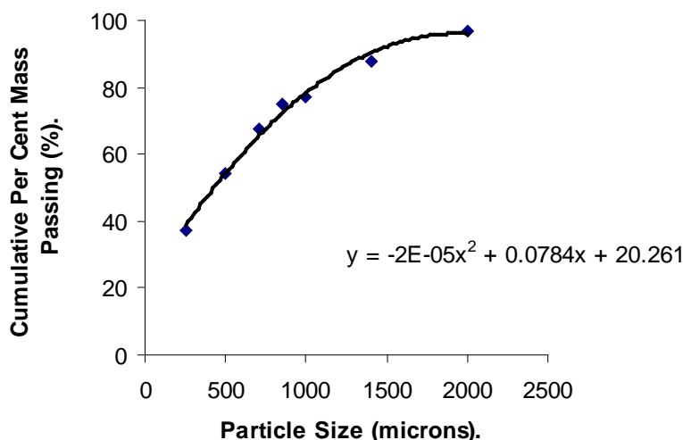
Figure 3: Lead-gold ore discharge particle size analysis.
