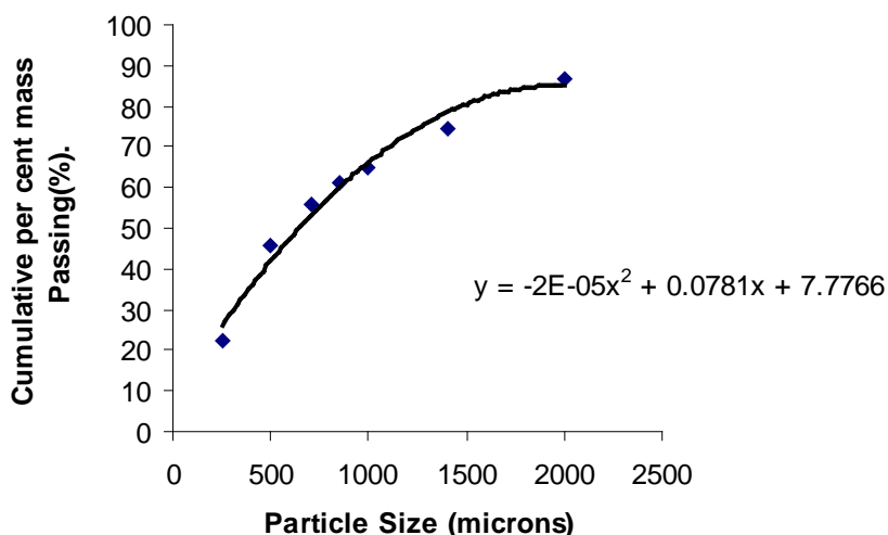
Figure 1: Particle size analyses of feed samples for grindability test
